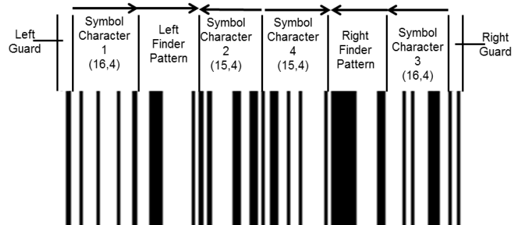
Figure 5.5.2.1-1. First group of GS1 DataBar symbols structure
